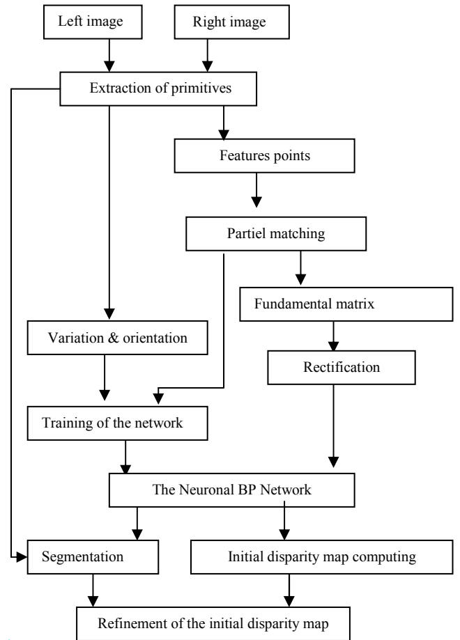
Figure2. Block diagram of the overall process.
