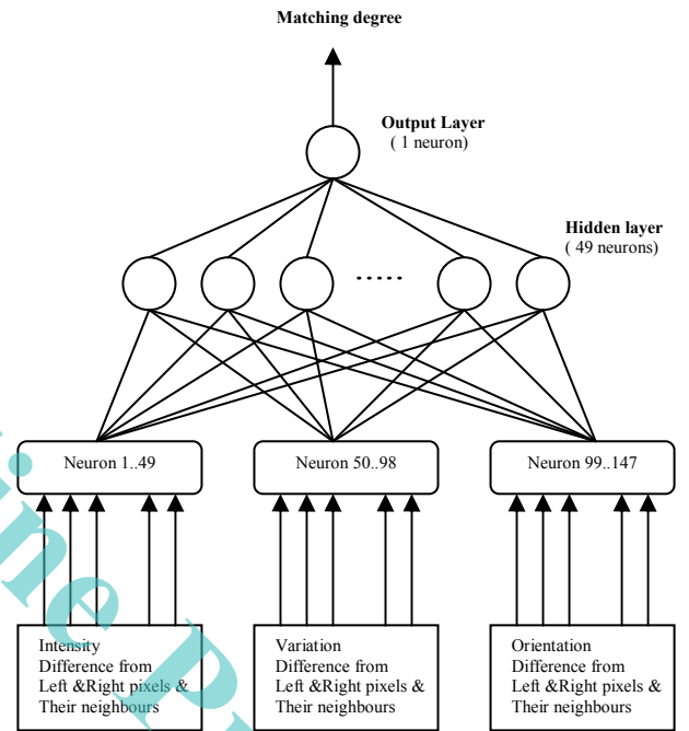
Figure 7. The BP neural network.
