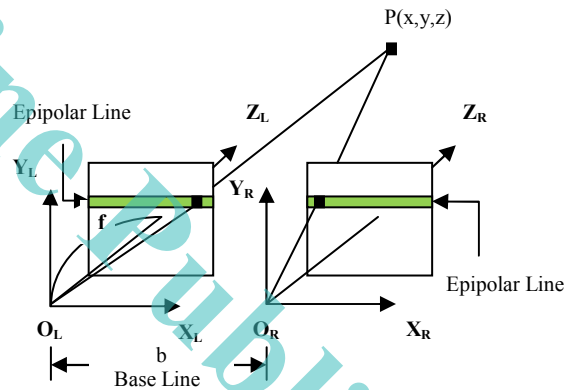
Figure 1. The parallel configuration in stereo vision.
